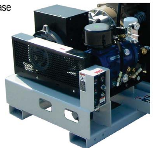
Tandem mounted compressor and generator.
